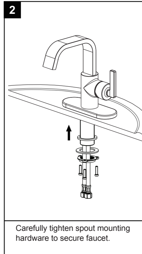
Install the faucet through the mounting hole.
